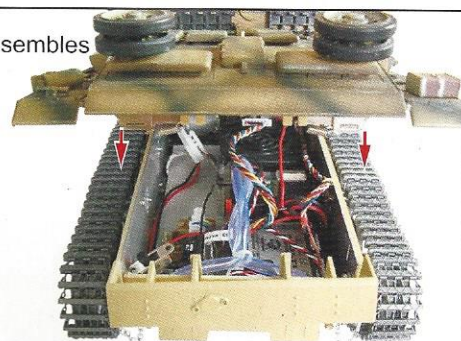
8. Opens the main body according to the arrow
